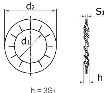
Type J, with internal teeth
