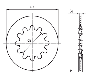
Type J, With internal teeth
